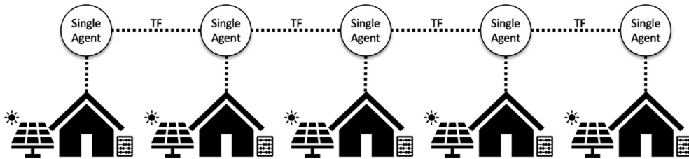
Fig. 3. Independent Learners with Transfer Learning topology.
