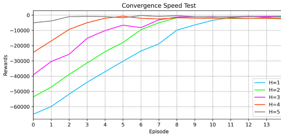
Fig. 7. Convergence speed.
